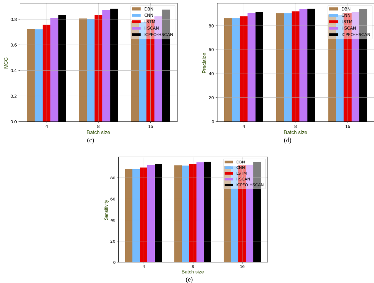
Fig. 7: Comparative estimation of detected model for given dataset over classical methods concerning (a) Accuracy, (b) FDR, (c) MCC, (d) Precision, (e) Sensitivity
