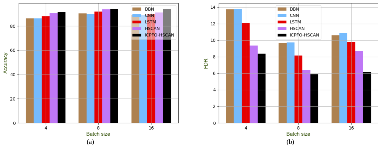
Fig. 6: Comparative estimation of the detected model for the given dataset over classical algorithms concerning “(a) Accuracy, (b) FDR, (c) MCC, (d) Precision, (e) Sensitivity”
